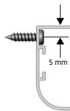
Screw Top Fix
