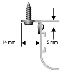
Screw Face Fix
